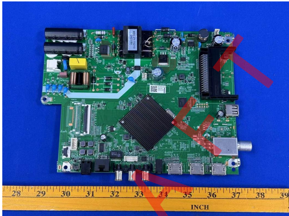
Internal Photo without DVB-S/S2 interface
